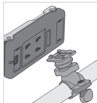
6 - Fitting of support in the mounting system
